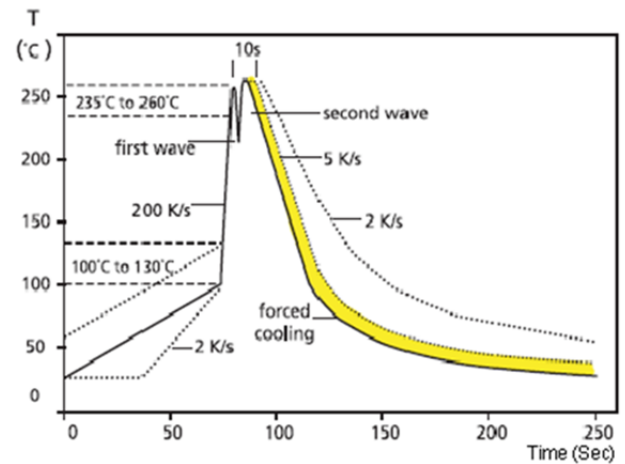
Recommended double-wave Soldering Profile
